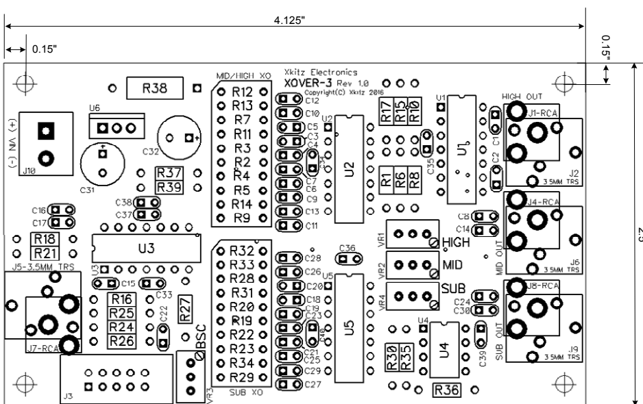
Figure 1. PCB Parts Placement and Dimensions
