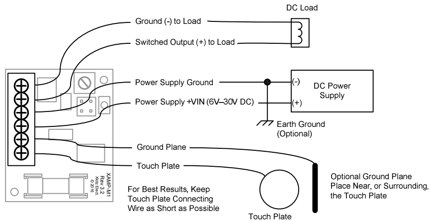
Figure 2. System Wiring Diagram
