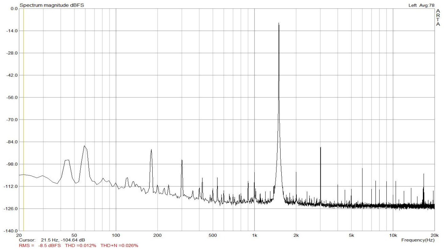
Figure 3. 2.83V into 8 Ohms (1W) , THD=0.012% THD+N=0.026%
