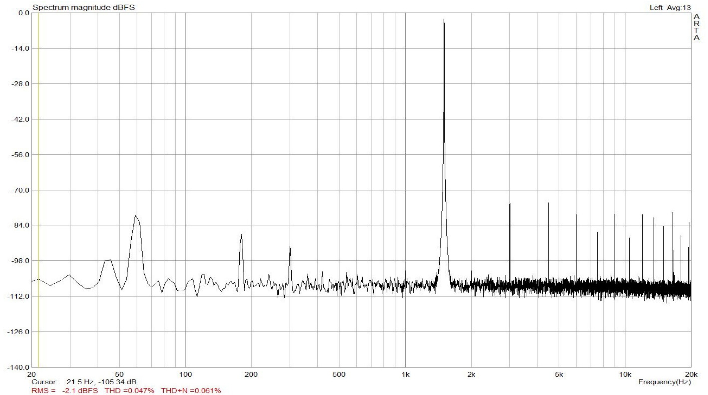
Figure 4. Full Output into 8 Ohms, THD=0.047% THD+N=0.061%
