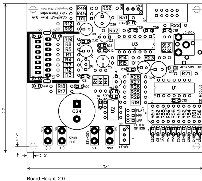
Figure 1. PCB Parts Placement and Dimensions
